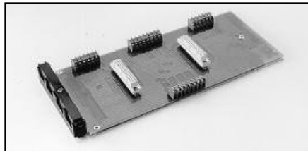
Model 7012-ST: Extra quick disconnect screw terminal board. One 7012-ST is included with each 7012-S.
