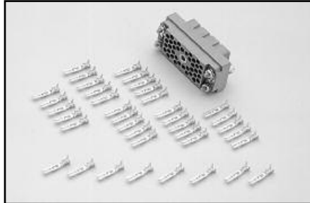
Model 7078-MTR: 38-pin bulkhead mount receptacle with 40 contacts for custom interface and patch panels compatible with 7078-MTC and 7078-KIT. Requires 7078-HCT; recommend 7078-CIT.
