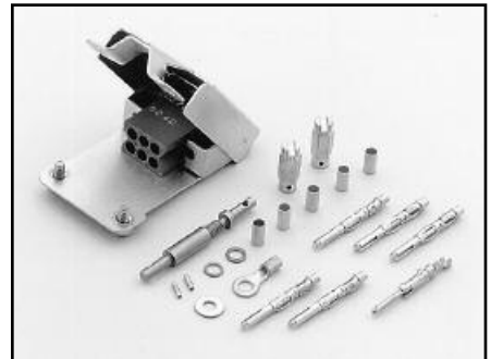
Model 7152-KIT: 6-pin plug assembly with strain relief and contacts for assembly of custom cable and harnesses compatible with Model 7152 4×5 Low Current Matrix Card and 7152-MTR Mass Terminated Receptacle. Requires 7152-HCT; recommend 7074-CIT and 7074-HCT.
