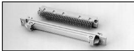
Model 7011-MTR: 96-pin male DIN connector with solder eyelets for bulkhead mount. Connects with the 7011-KIT-R and the 7011-MTC-2.
