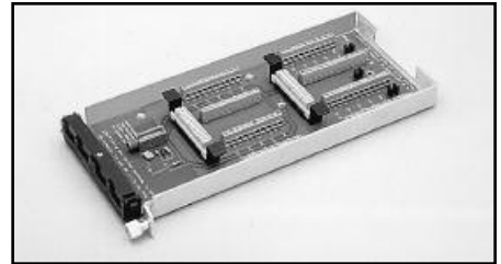
Model 7014-ST: Extra quick disconnect isothermal screw terminal board with cold junction sensor. One 7014-ST is included with each 7014.
