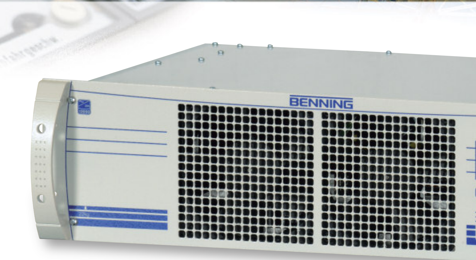
Fig. 8: 19" rectifier TEBECHOP 12000 I output voltage 220 V, output current 45 A
