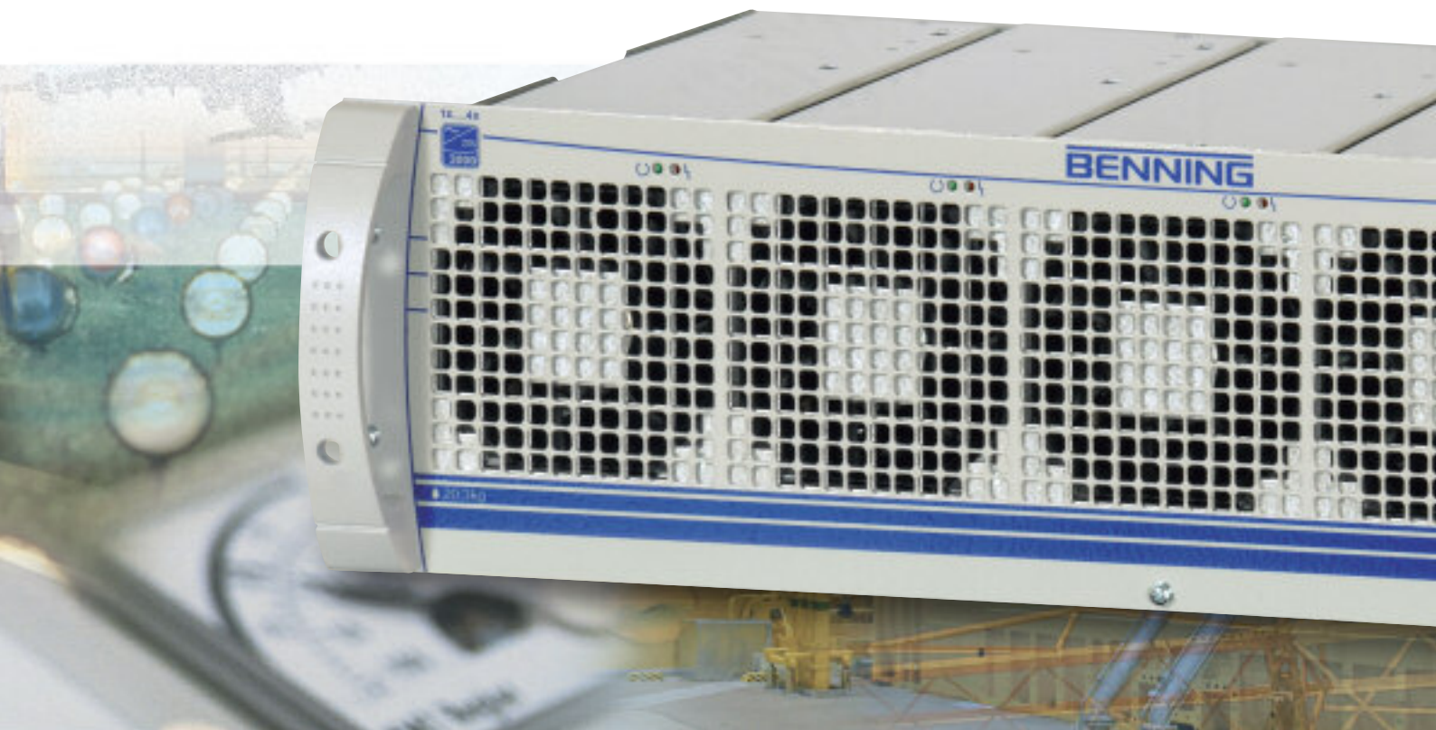
Fig. 7: 19" modular rectifier shelf with 4 modules TEBECHOP 3000 I and remote monitoring unit MCU 2500 output voltage 110 V, output current 80 A
