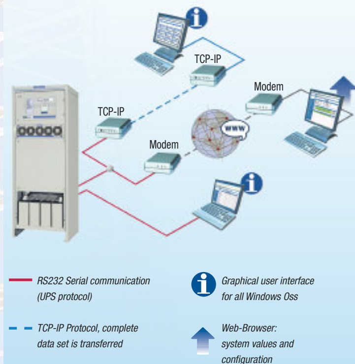
Fig. 10: Monitoring concept of the MCU 2500
