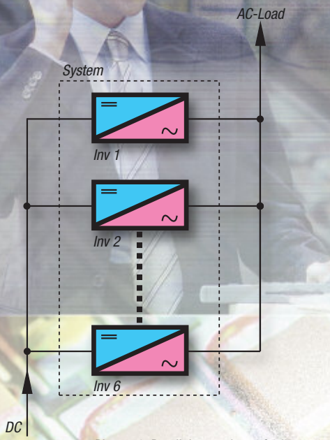
Picture 1: Parallel operations of 6 inverters
