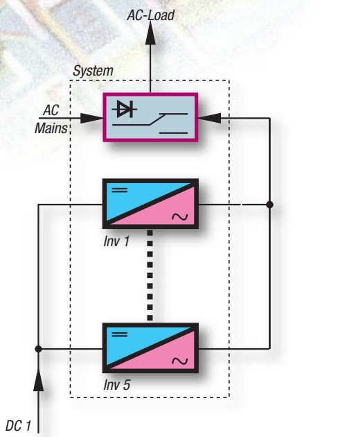
Picture 3: Parallel operation of 5 inverters and a static bypass
